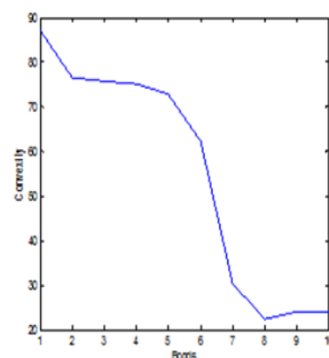
Figure- 4.3. Convexity.
