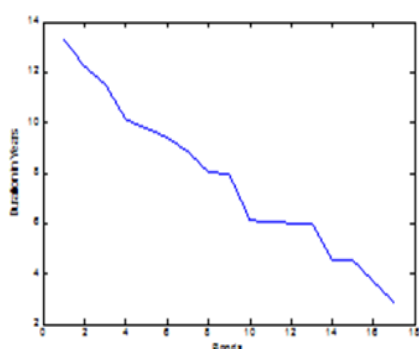
Figure-3.1. Duration.
