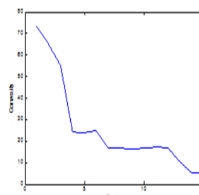
Figure-2.3. Convexity.
