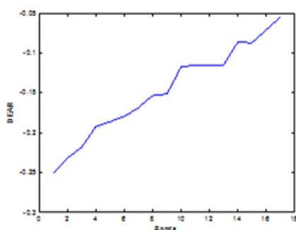
Figure-3.4. DEAR.
