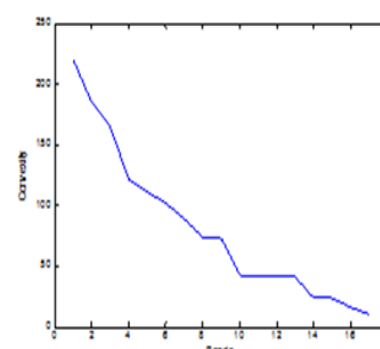
Figure-3.3. Convexity.
