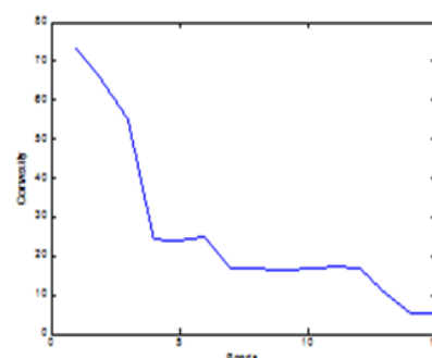
Figure-1.3. Convexity.
