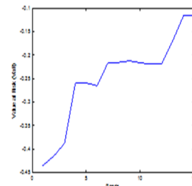
Figure-2.6. VaR.
